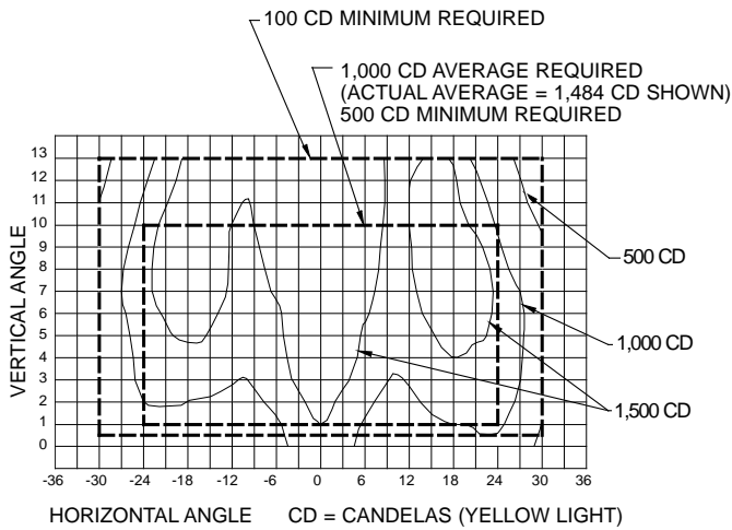
L-852G Runway Guard Light – Yellow
