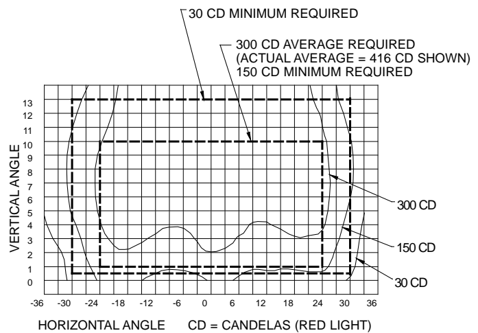
L-852S Stop Bar Light – Red
